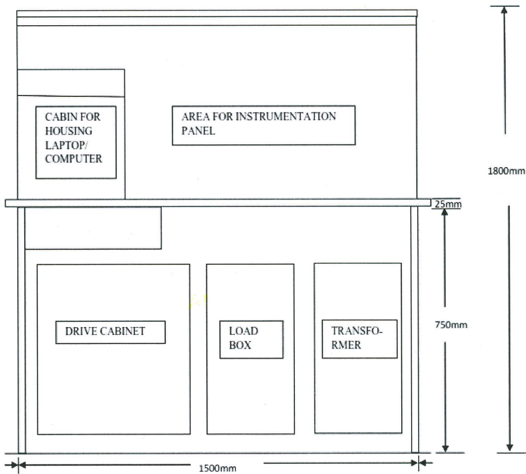
Fig.8 Layout of the wooden worktable-front view
