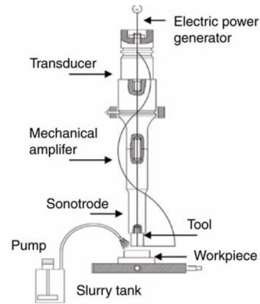
Figure 1. Ultrasonic Machine
