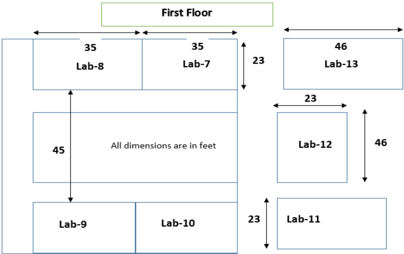
Layout for First Floor
